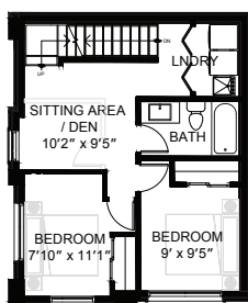
OPTIONAL 2 Bedroom with Sitting Area
